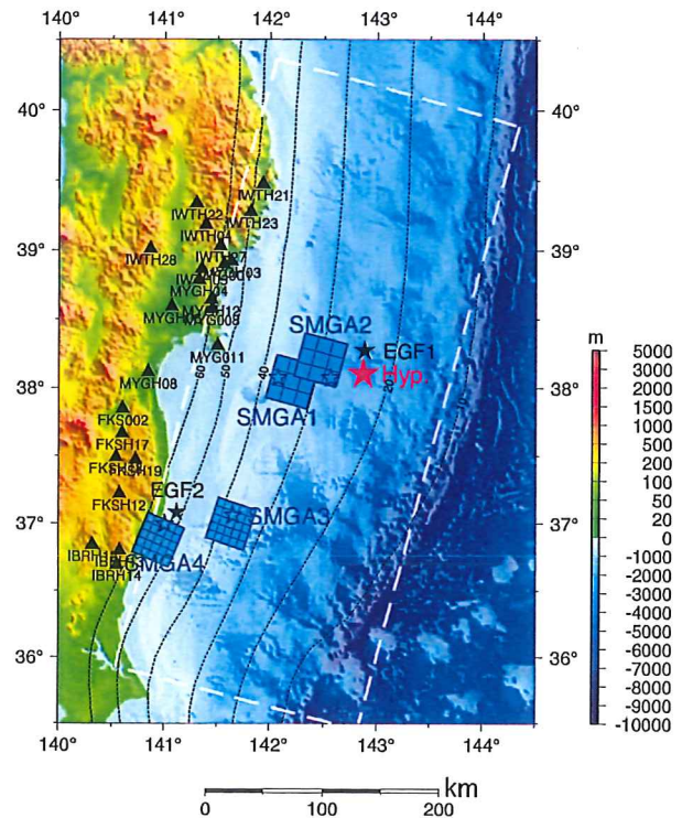
Fig. 6. The source model composed of four SMGAs shown in the map. The large and small solid stars indicate the epicenters of the mainshock and EGF events, both determined by JMA, respectively. The blue open stars represent the rupture starting points of SMGAs. Solid triangles indicate the strong motion stations used in the grid search. The broken rectangle indicates the source fault plane of the 2011 Tohoku earthquake, from Suzuki et al. (2011). The broken contour lines represent the depth of plate interface from Nakajima and Hasegawa (2006) and Nakajima et al. (2009) with an interval of 10 km.
