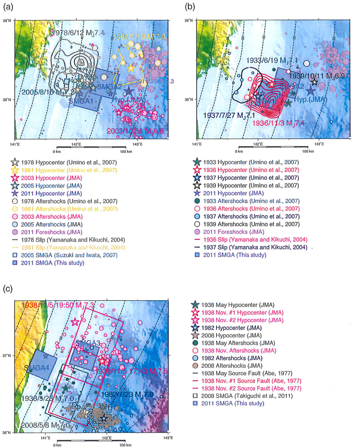
Fig. 9. (a) Comparison of SMGA1 and SMGA2 with the source regions of 1978, 1981, 2003, and 2005 events in the Miyagi-oki region. The contours show the slips of the 1978 and 1981 events estimated by Yamanaka and Kikuchi (2004) projected on the map, and the contour interval is 0.4 m. Filled stars indicate the hypocenters of the mainshocks of each sequence, and circles indicate their aftershocks by Umino et al. (2007) and JMA. (b) Comparison of SMGA1 and SMGA2 with the source regions of 1936 and 1937 events in the Miyagi-oki region. The contours show the slips of the 1936 and 1937 events estimated by Yamanaka and Kikuchi (2004) projected on the map. The contour intervals for the 1936 and 1937 events are 0.4 m and 0.3 m, respectively. (c) Comparison of SMGA3 and SMGA4 with the source regions of three M 7-class events in 1938 in the Ibaraki region. The rectangles correspond to the map projections of source fault planes obtained for three events in 1938 by Abe (1977). Filled stars indicate the hypocenters of mainshocks of each sequence, and circles indicate their aftershocks by JMA.
