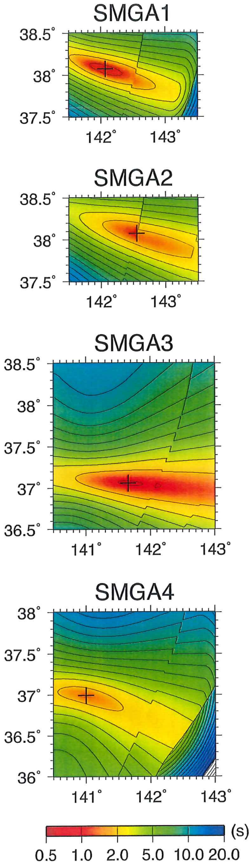
Fig. 4. Distributions of RMS residuals estimated by the grid search method for locating the rupture starting points of SMGAs. The contour interval is 1 s. The cross indicates the minimum value.
