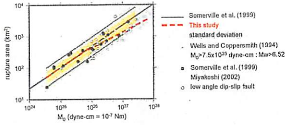
Fig. 1. Rupture area versus seismic moment. Thick broken line shows the empirical relation obtained in this study. Shadow ranges \sigma (standard deviation). Thin solid lines show factor of 2 and 1/2 for the average.
